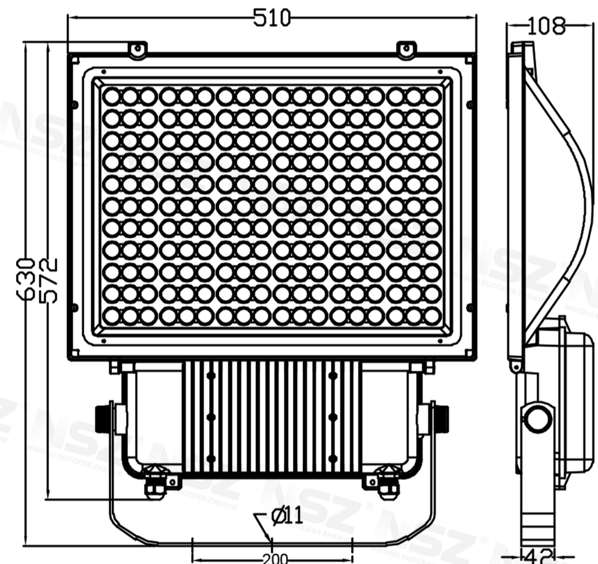
ZY-2004SMD 100W
