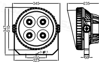
ZY-2078G-160W/200W
