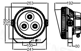
ZY-2078G-60W/90W
