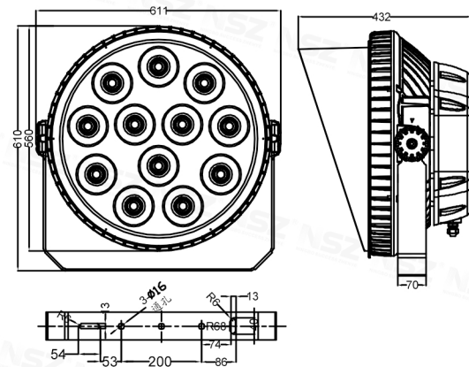
ZY-2078G-500W/600W
