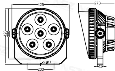
ZY-2078G-240W/300W
