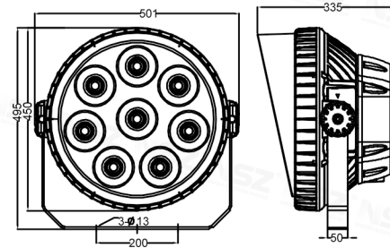
ZY-2078G-360W/400W
