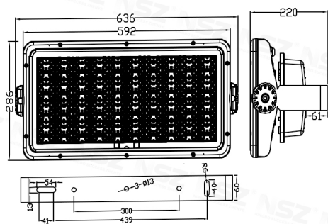
ZY-2086-500W
