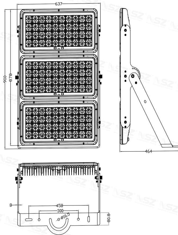
ZY-2086-1200W/1500W
