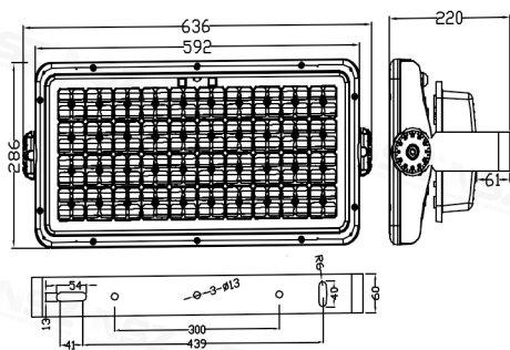
ZY-2086-400W
