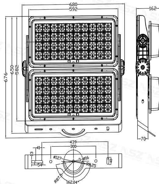
ZY-2086-800W/1000W
