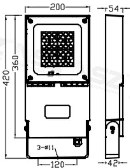
ZY-2088F-50W
