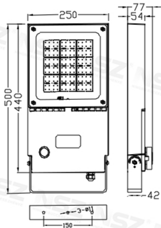
ZY-2088F-100W
