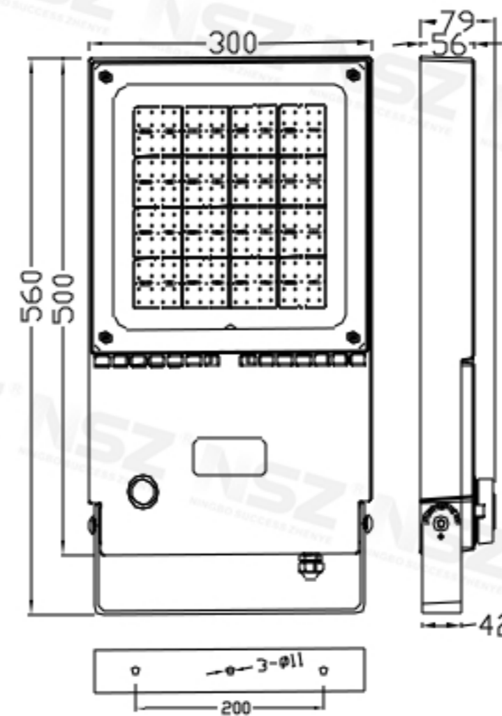
ZY-2088F-200W
