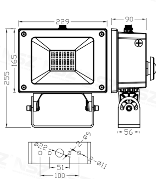
ZY-2089B SMD 50W
