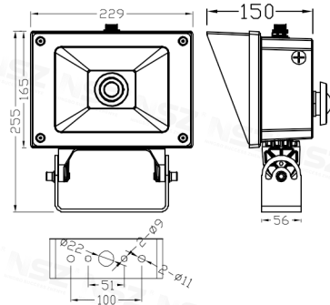
ZY-2089B Reflection cup 50W
