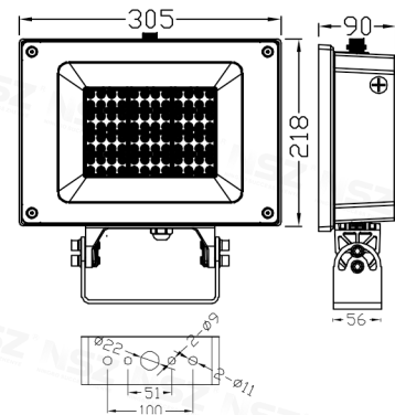
ZY-2089B SMD LENS 60W
