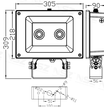
ZY-2089B COB 100W
