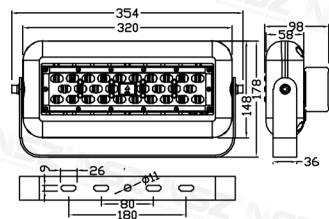
ZY-2091 30W/50W/60W
