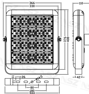
ZY-2091 160W/180W/200W
