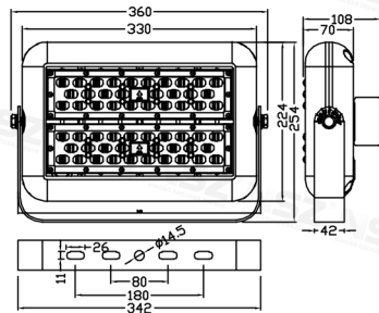
ZY-2091 80W/100W
