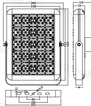
ZY-2091 240W/250W/300W
