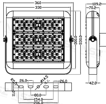
ZY-2091 120W/150W
