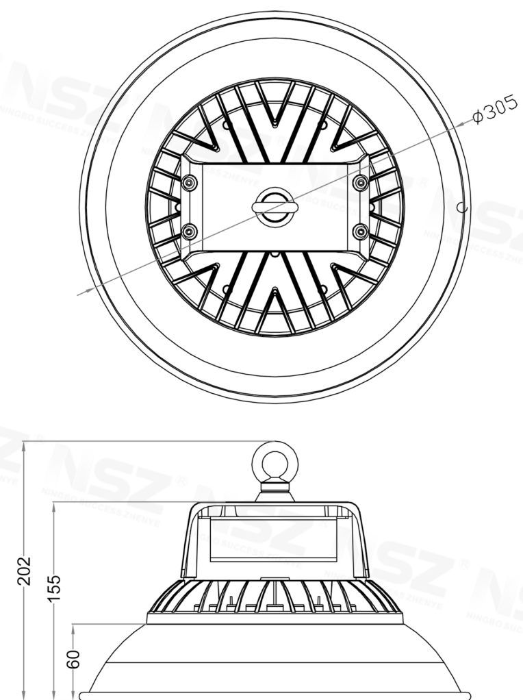
ZY-8001DC 50W
