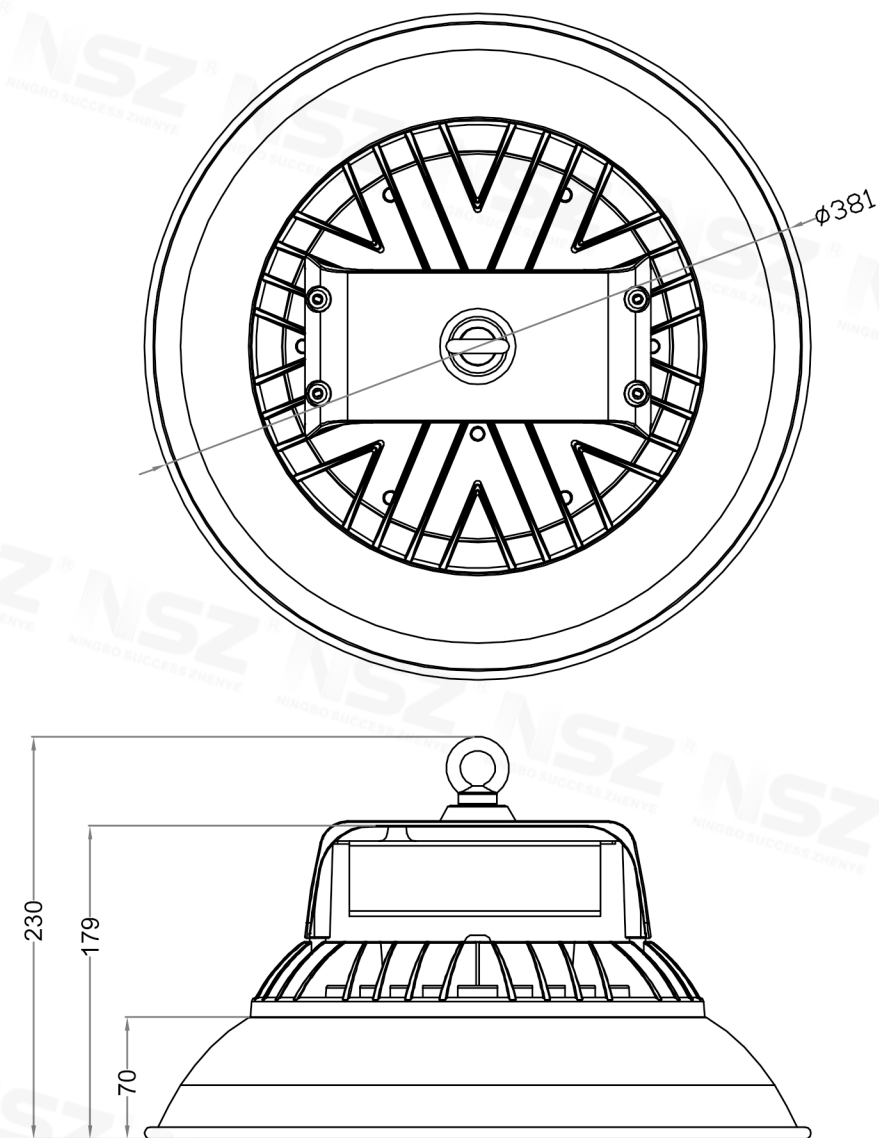
ZY-8001DC 100W
