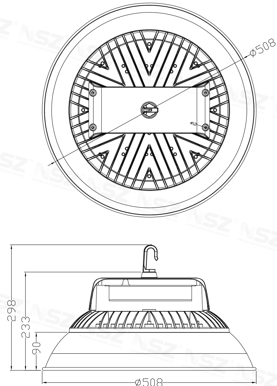
ZY-8001DC 200W
