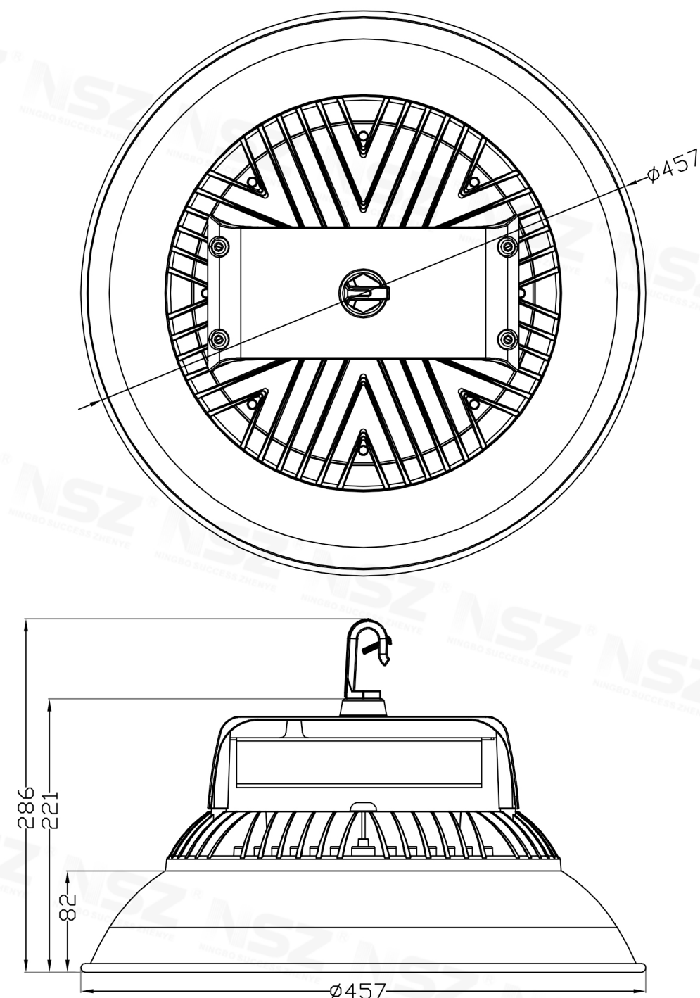
ZY-8001DC 150W
