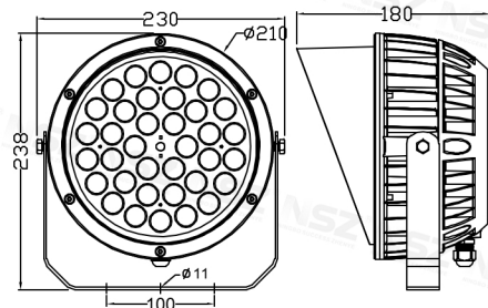
ZY-9006 50W/80W/100W With shield
