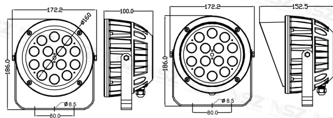
ZY-9006 6W/9W/12W/18W With shield and ground insert
