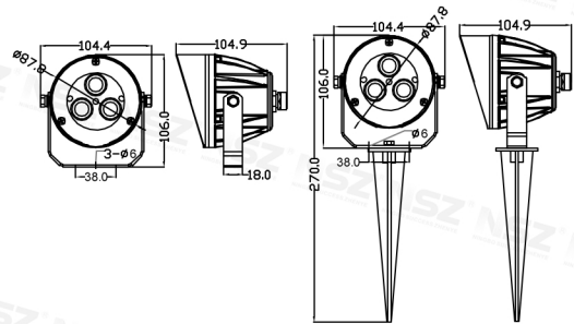
ZY-9006 3W/6W With shield and ground insert
