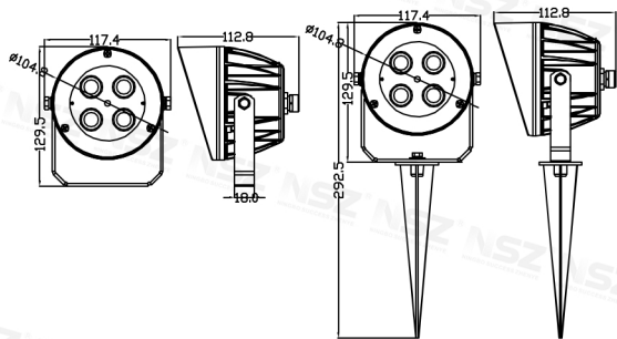
ZY-9006 6W/9W With shield and ground insert
